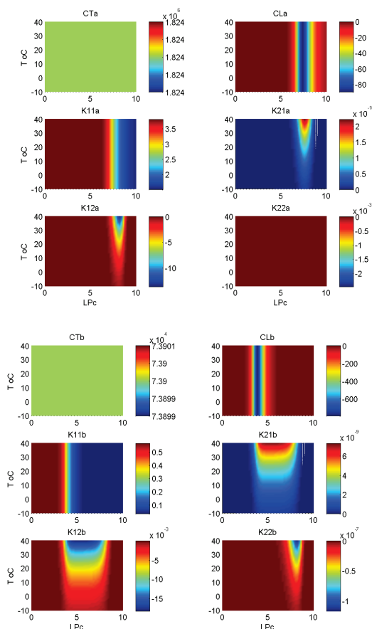
Figure 2. PDE coefficients C_T , C_{LPc} , K_{ij} as functions of LPc and T calculated from the provided HAMSTAD benchmark no.1 material properties for the load bearing (a) and insulation (b) material
