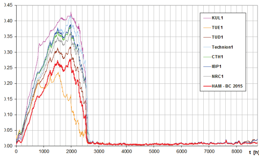
Figure 4. The average moisture content in the insulation.
