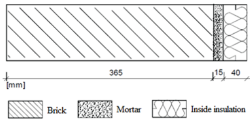
Figure 16. Geometry of the benchmark 5.
