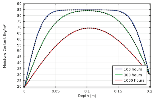
Figure 6. Moisture content [kg/m 3 ] related to the depth [m] measured from the outside after 100 hours, 300 hours and 1000 hours, where the colored graphs are the results of our model and the dotted graphs are the analytical solutions.
